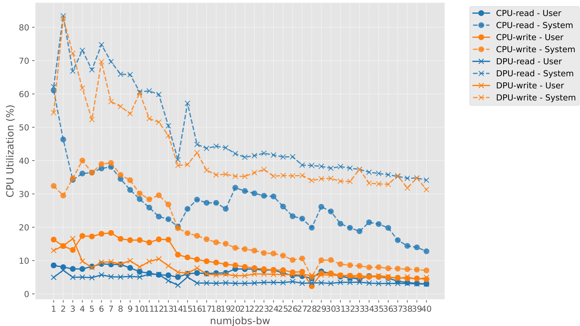
CPU Utilization vs numjobs-bw (CPU vs DPU)
